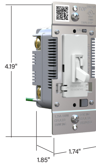
Depth (Into Wallbox) = 1.57" TSDL153PW
