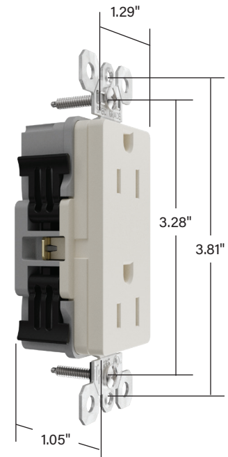
Depth (into Wallbox) = 1.05" TR26342DVSLA
