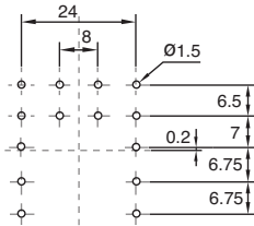
Dimensions [mm]
