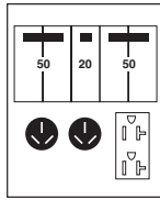
Fig. J U002C (2) 10-50R, 5-20R2
