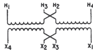
Wiring Diagram for Low Voltage Loads
