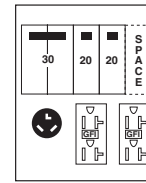
Fig. G U666C010 10-30R, (2) 5-20R2GFCI
