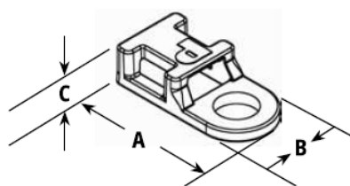
TA1 Mount
