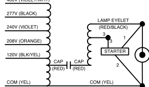
Wiring Diagram 2
