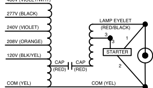
Wiring Diagram 2
