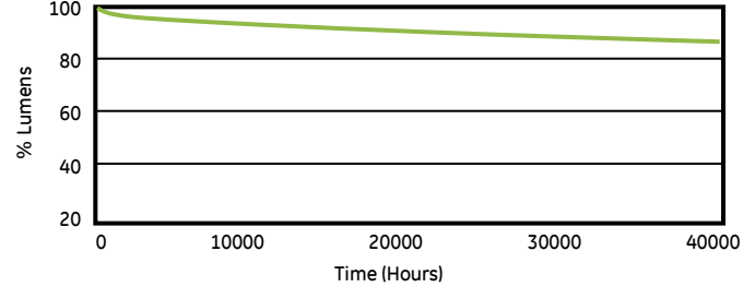
Lumen Maintenance
