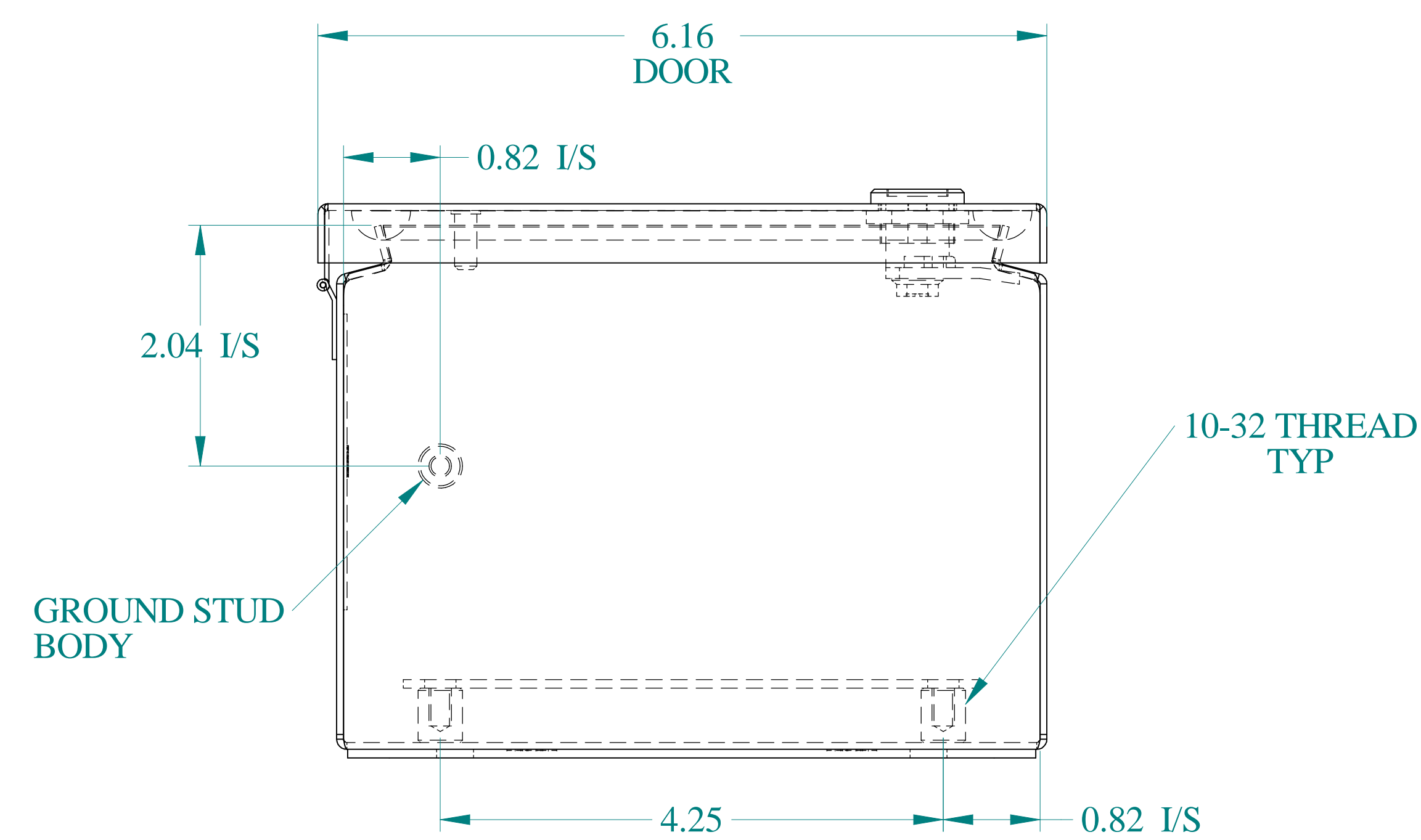
BOTTOM VIEW
