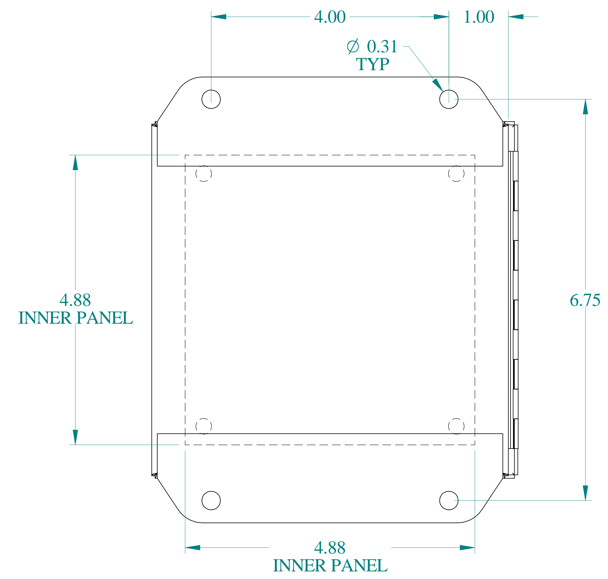
BACK VIEW
