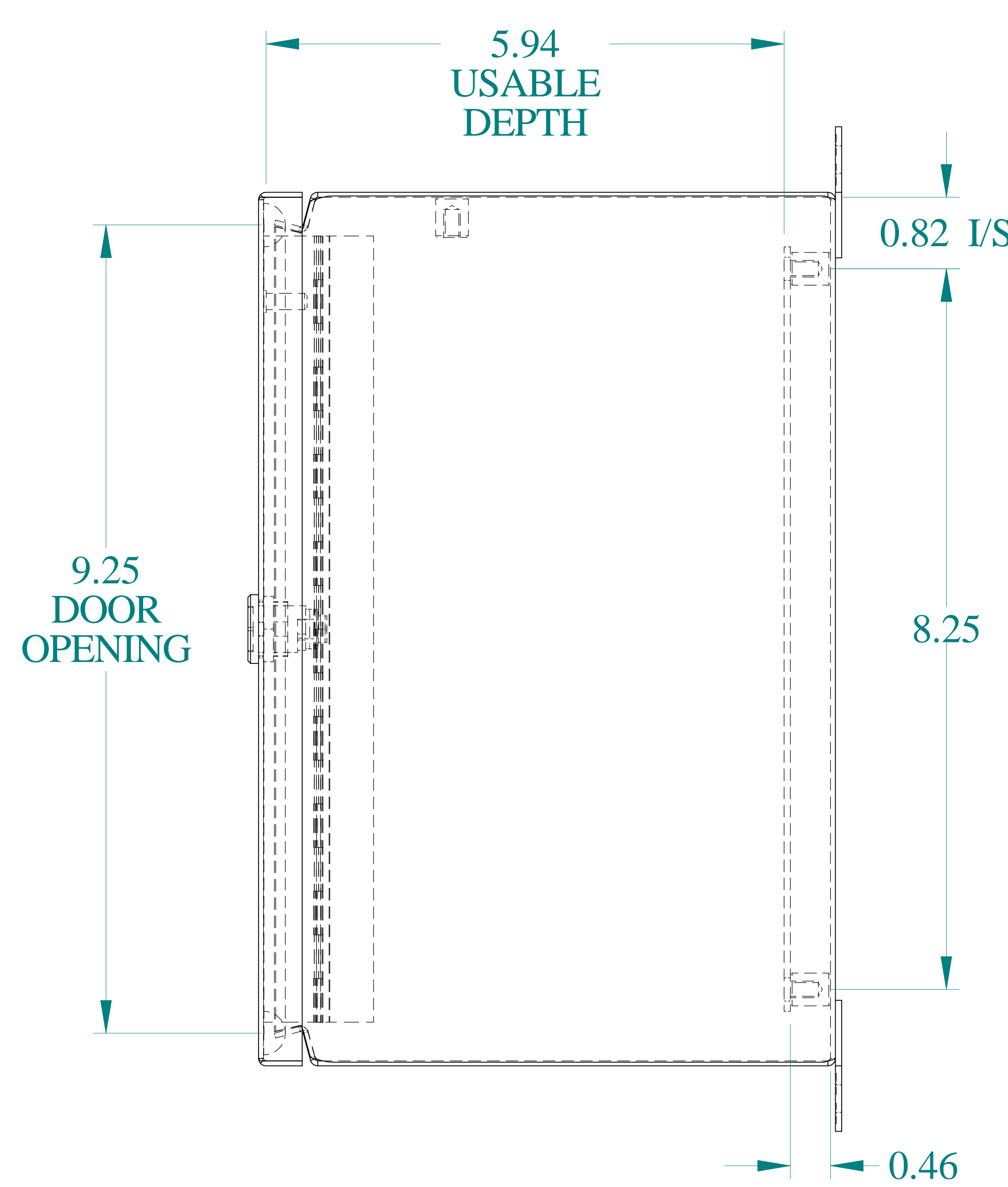
SIDE VIEW
