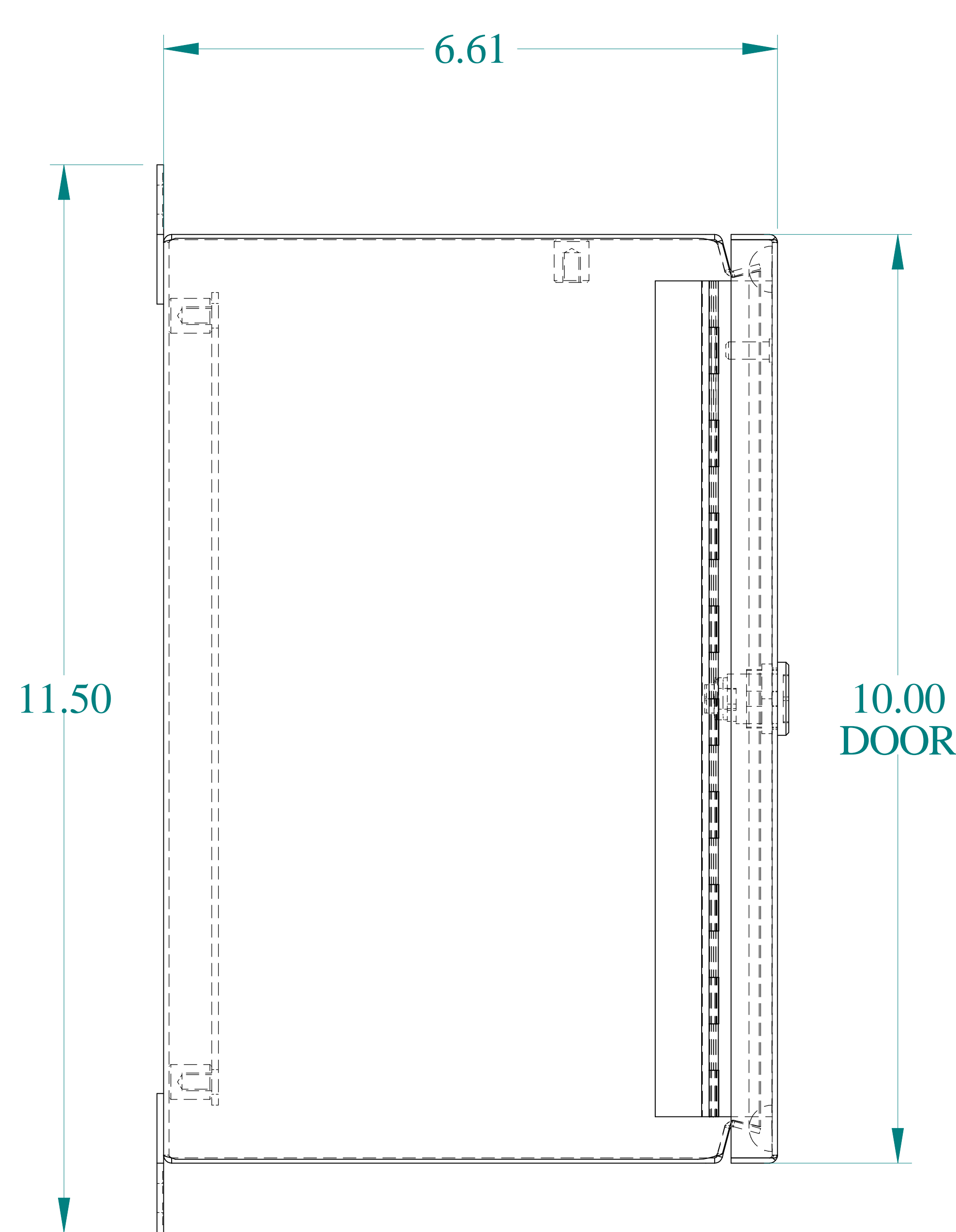
SIDE VIEW
