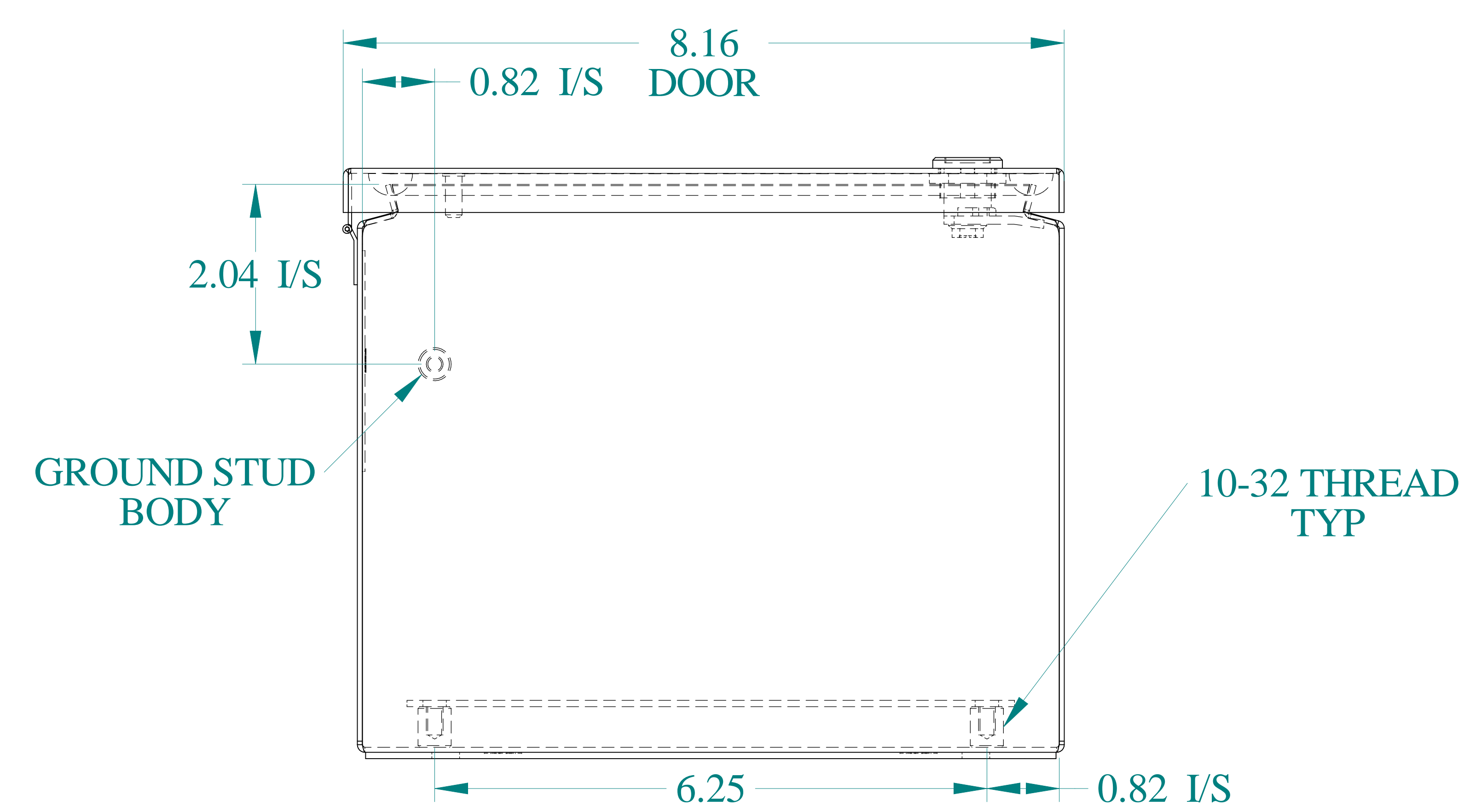
BOTTOM VIEW
