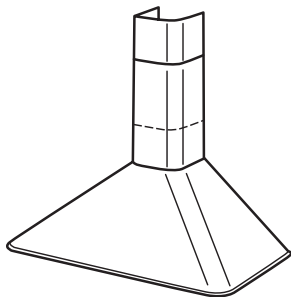
6" Round Duct — Internal Blower High — 290 CFM, 5.5 Sones Normal — 135 CFM, 0.5 Sones
