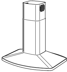
6" Round Duct — Internal Blower High — 480 CFM, 9.5 Sones Low — 230 CFM, 3.0 Sones
