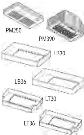
PM250 7" Round Duct — Internal Blower 250 CFM — 8.0 Sones PM390 6" Round Duct — Internal Blower 390 CFM — 6.0 Sones
