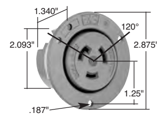
Dimensions for 20 Amp Flanged Outlet
