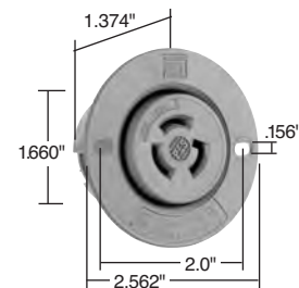
Dimensions for 15 Amp Flanged Outlet
