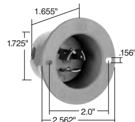
Dimensions for 15 Amp Flanged Inlet
