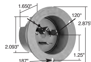
Dimensions for 20 Amp Flanged Inlet
