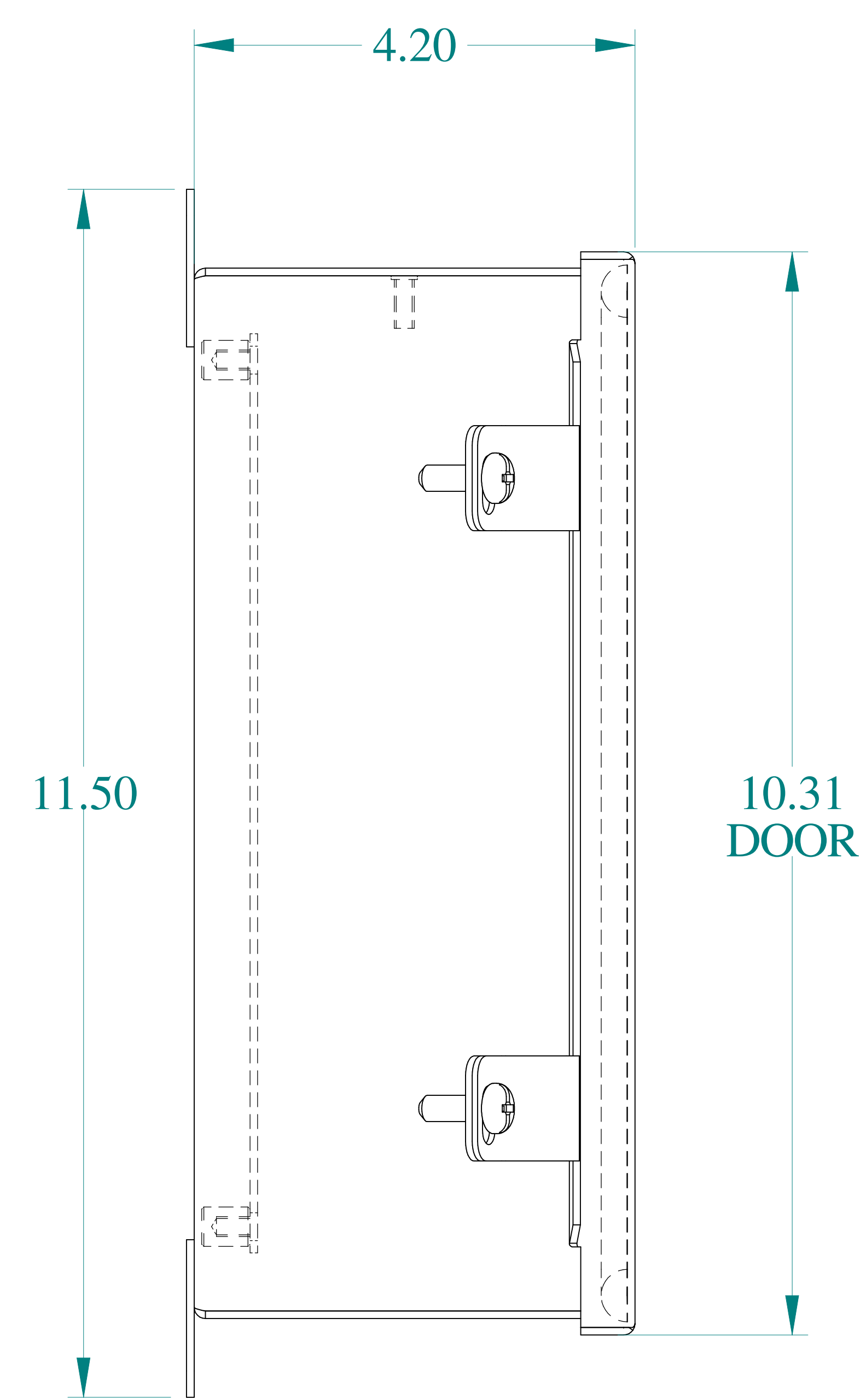
SIDE VIEW
