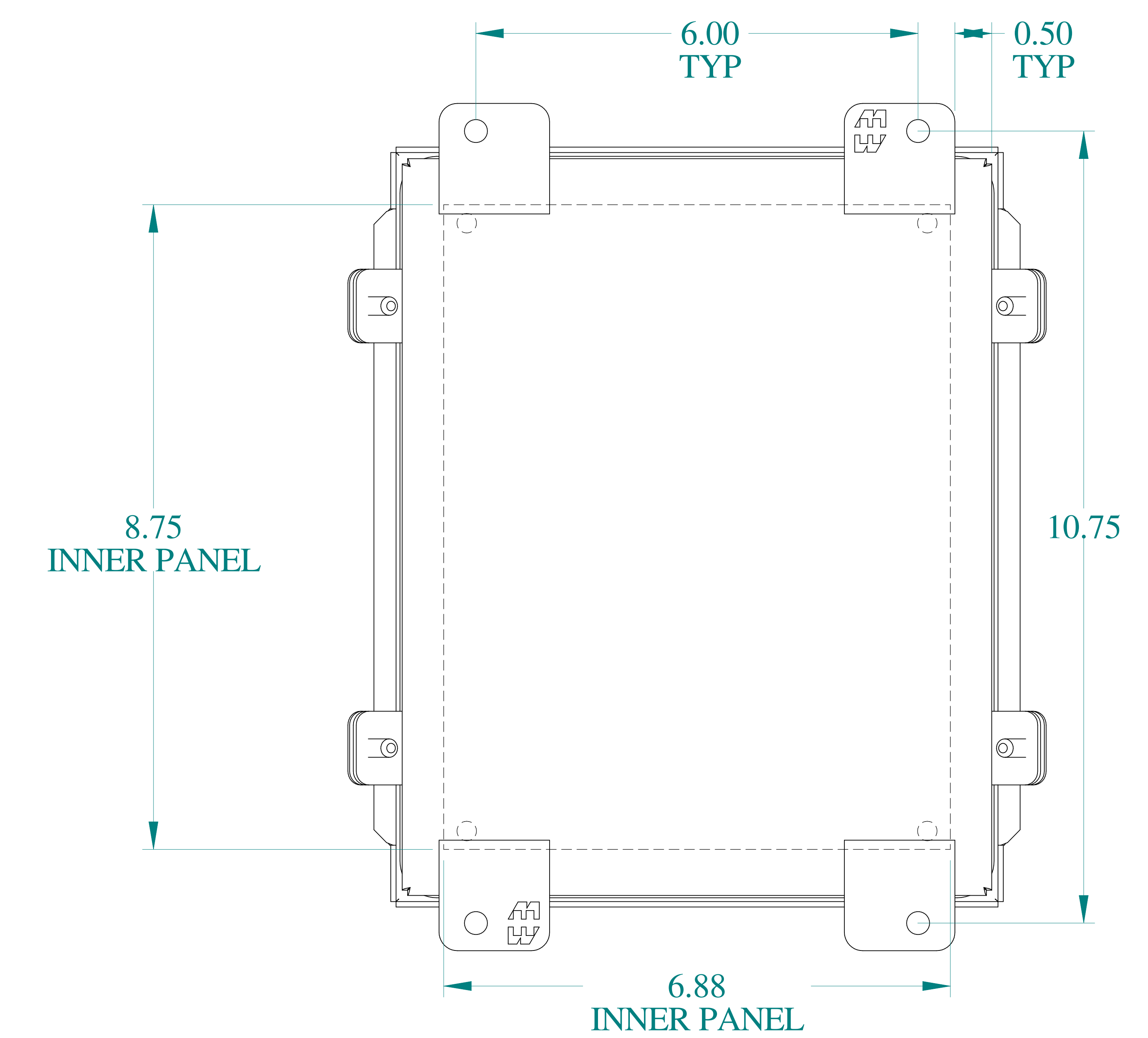
BACK VIEW
