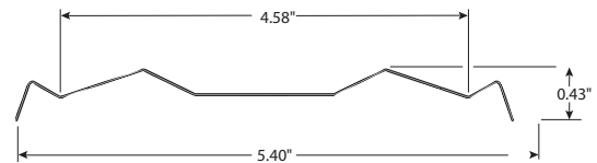
6-inch Reflector
