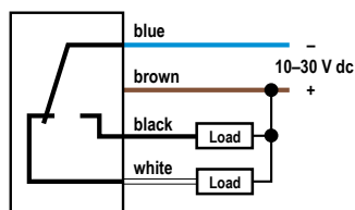
NPN Models
