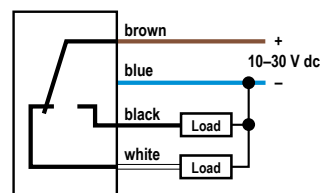
PNP Models
